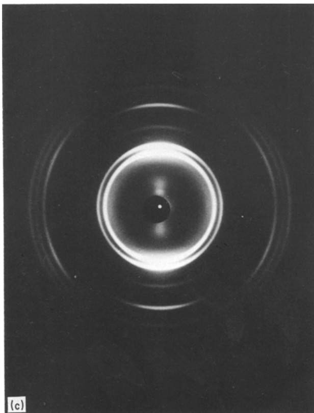
Figure 10 Wide-angle X-ray diffraction patterns of a ribbon-shaped polyethylene fibre (HifaxB) spun at a polymer concentration of 1.5 wt % at a spinning temperature of 215°C with a spinning speed and winding speed of 100 m min -1 . (a) Incident X-ray beam along the fibre axis, flat fibre surface vertical; (b) incident X-ray beam flat-on, fibre axis vertical; (c) incident X-ray beam edge-on, fibre axis vertical.
